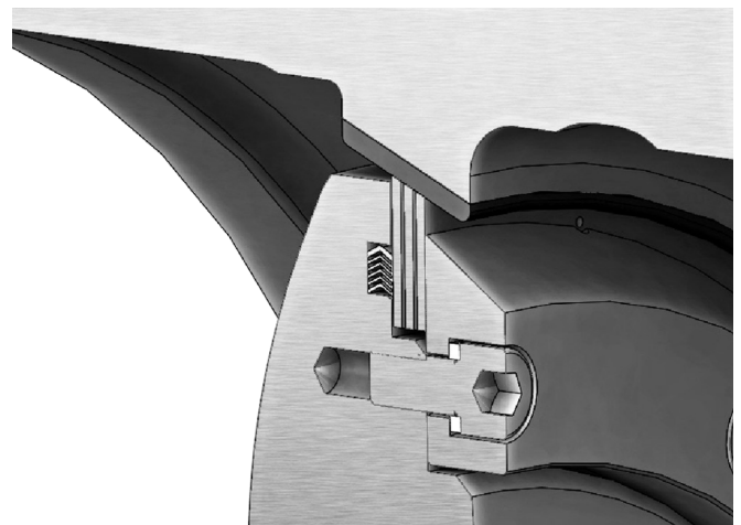
After Sealing Contact
