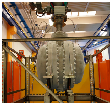
Steam Cracking Blow Down (Ground-level Smokeless Torch), Italy
